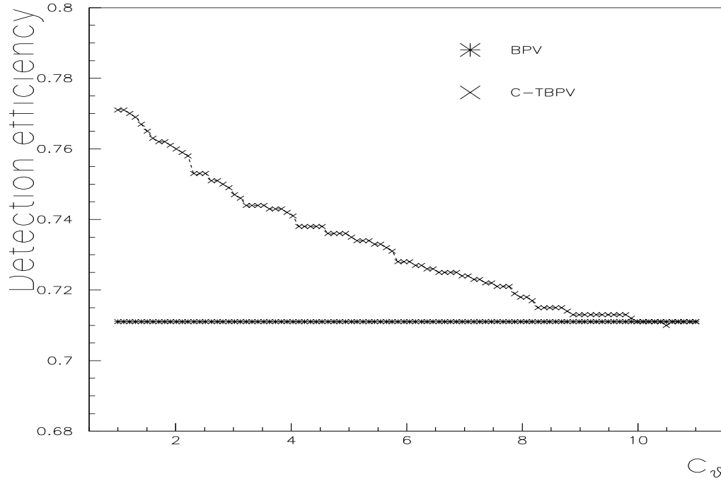
Figure 3: Jump detection efficiency for the model (3.1) in the presence of a single jump, as a function of the threshold parameter c_{\vartheta} .
